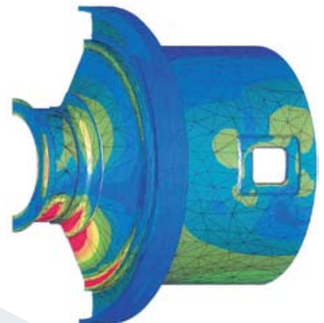
FEA on a large diameter SAG Mill
