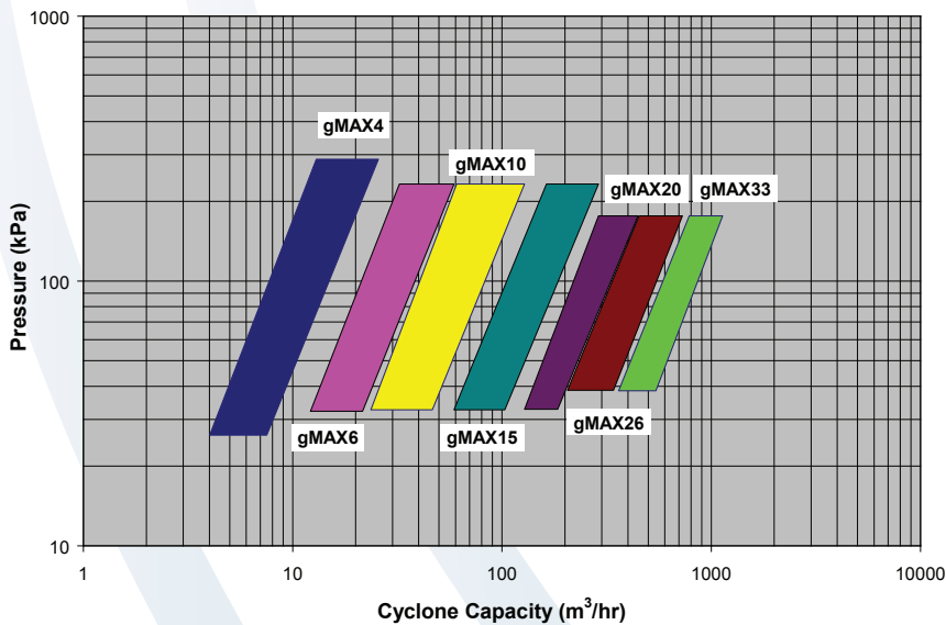
FLSmidth Krebs gMAX Capacity Curves- Metric Units
